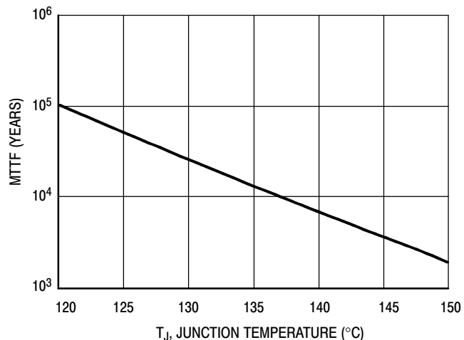
NOTE: The MTTF is calculated with V DC = 5 Vdc, I DC = 250 mA Figure 3. MTTF versus Junction Temperature
